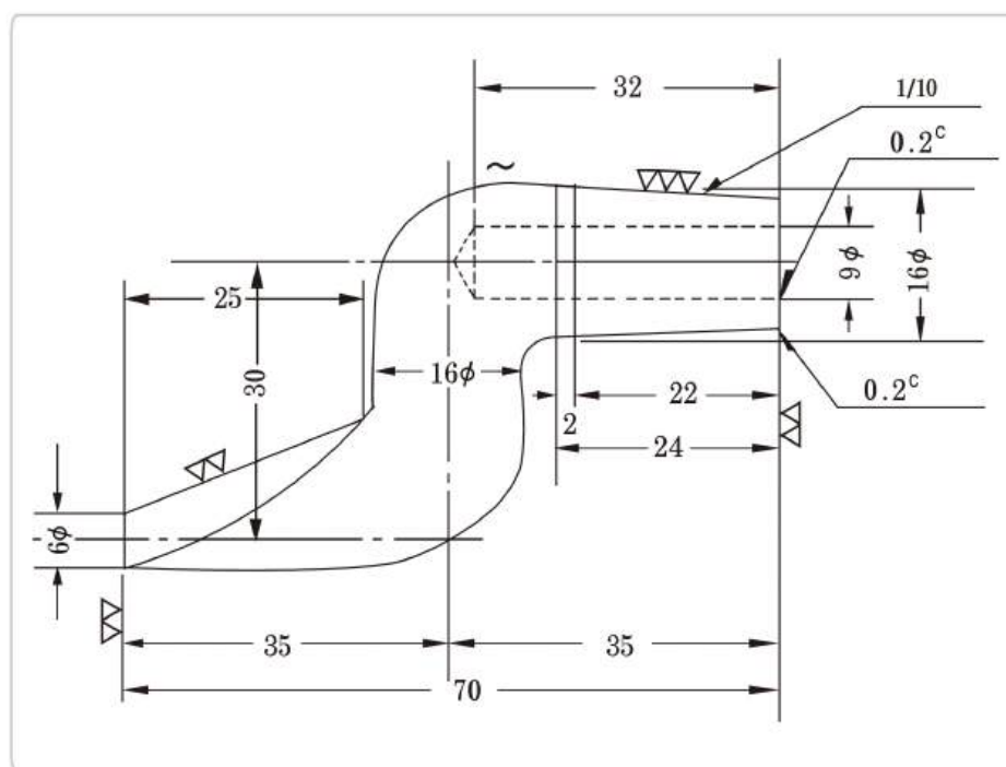
EK-C-2-2 中彎 Medium Bent Tip Two Point Bent
