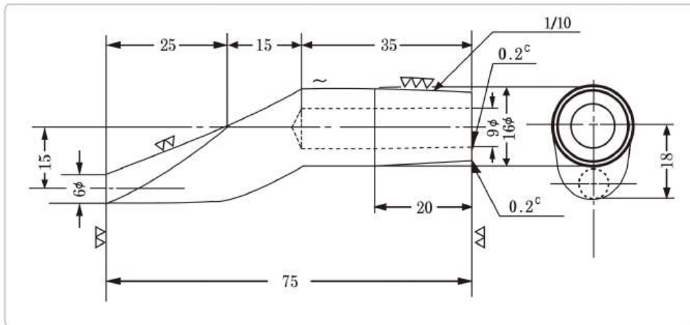
EK-C-1-2 小彎 Small Bent Tip One Point Bent
