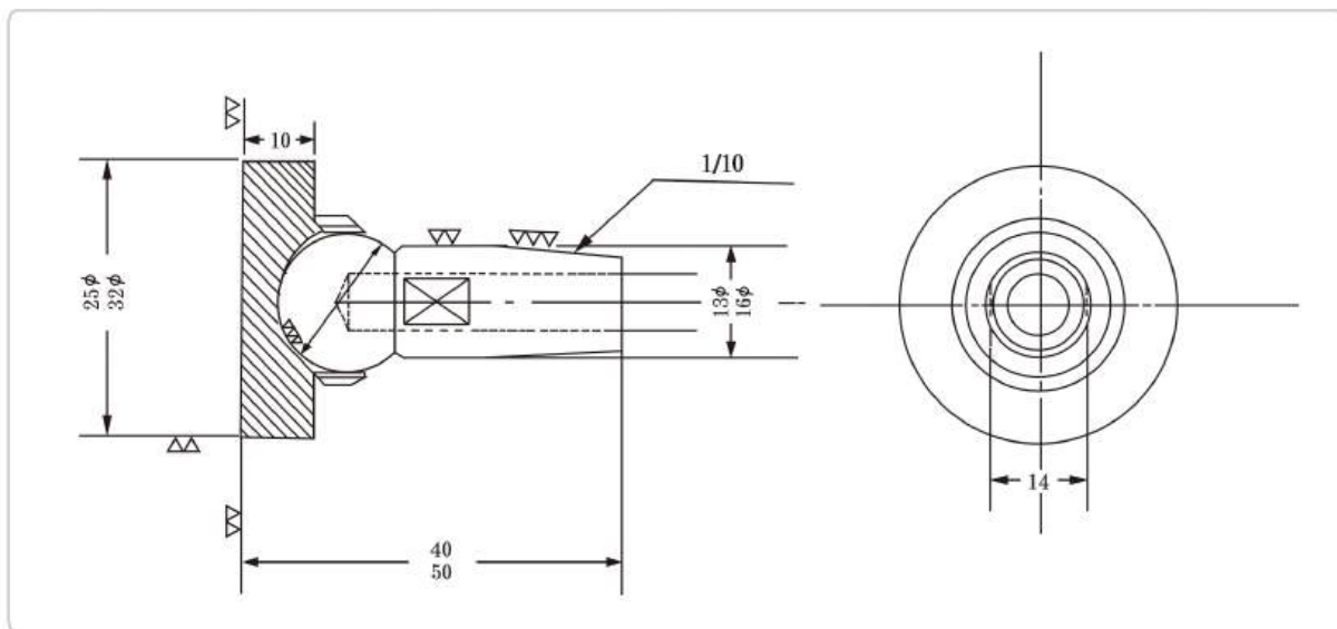
EK-C-2-2 中彎 Medium Bent Tip Two Point Bent
