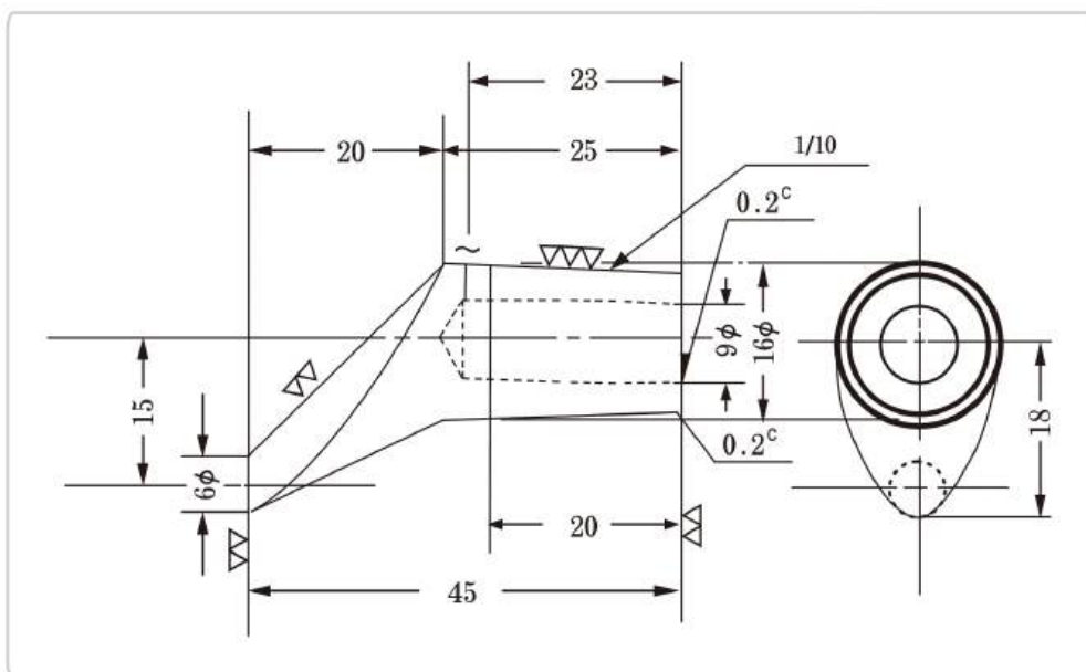
EK-C-2-3 大彎 Big Bent Tip Two Point Bent(long)
